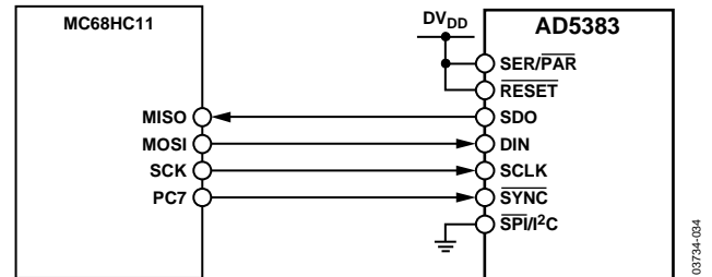
Figure 34. AD5383-to-MC68HC11 Interface
