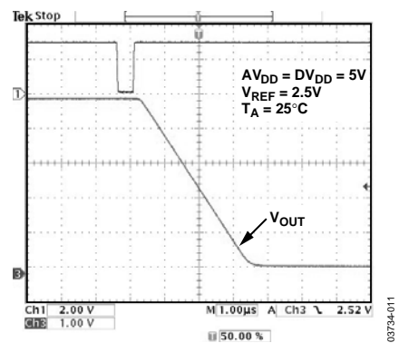
Figure 11. Slew Rate with Boost Off
