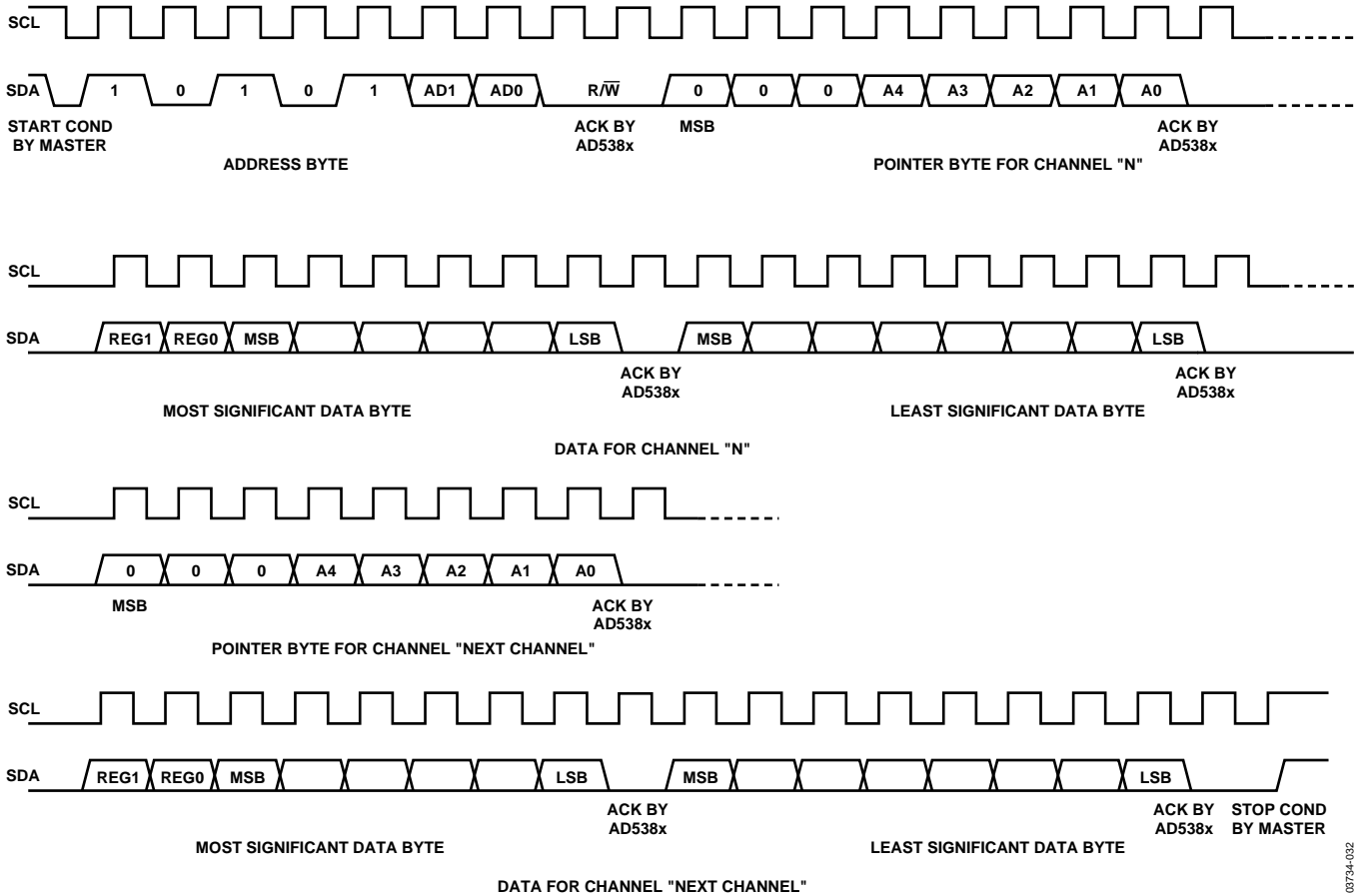
Figure 32. 3-Byte, I 2 C Write Operation
