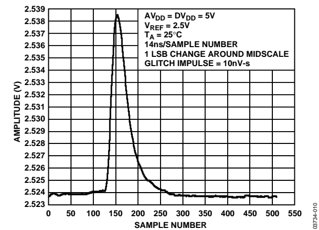
Figure 10. AD5383-5 Glitch Impulse
