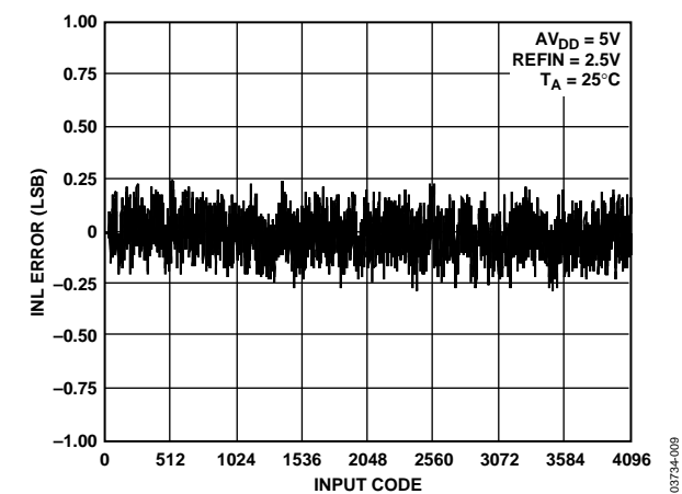
Figure 9. Typical AD5383-5 INL Plot
