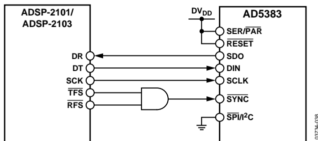
Figure 38. AD5383-to-ADSP-2101/ADSP-2103 Interface
