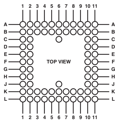
74-LEAD CSPBGA BALL CONFIGURATION
