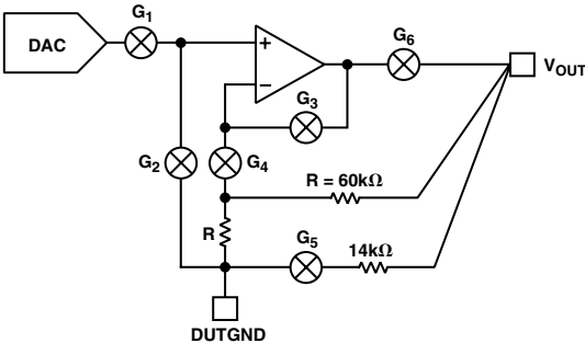
Figure 4. Block Diagram of AD7841 Output Stage
