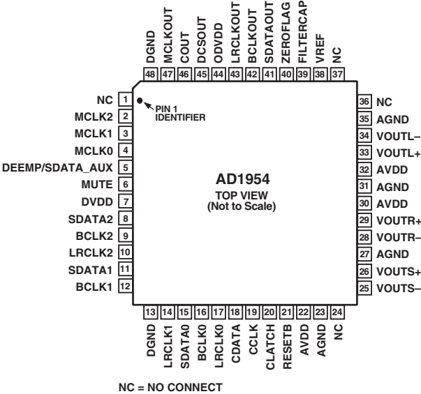
48-LEAD LQFP
