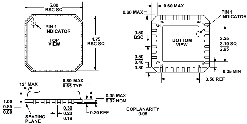
Figure 57. 32-Lead Lead Frame Chip Scale Package [LFCSOP] 5 mm × 5 mm Body (CP-32-2) Dimensions shown in millimeters
