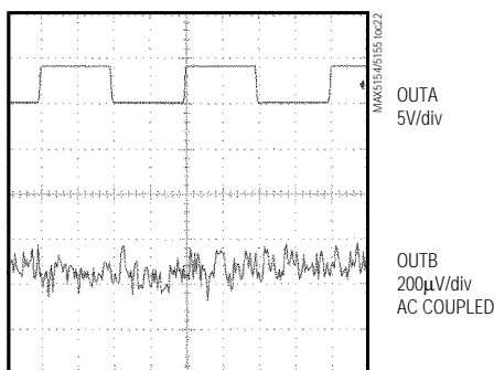
V_{REF} = 2.048V , GAIN = +2V/V, CODE = 1FFE HEX
