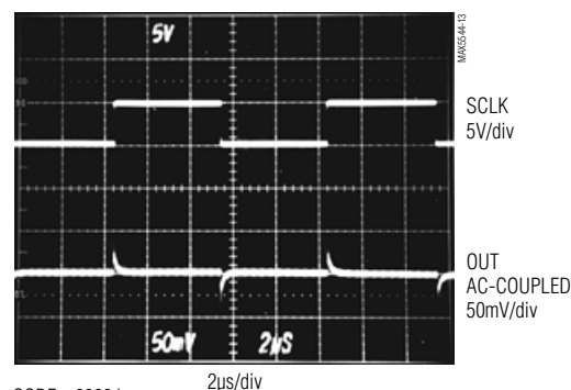
DIGITAL FEEDTHROUGH
