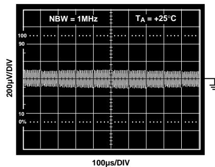
Figure 10. Broadband Noise
