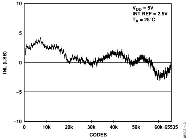
Figure 12. INL AD5668-2/AD5668-3
