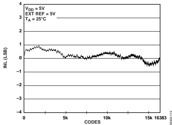
Figure 13. INL AD5648-2
