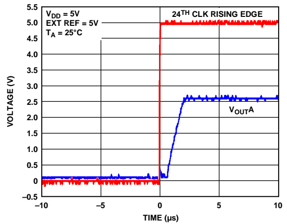
Figure 40. Exiting Power-Down to Midscale
