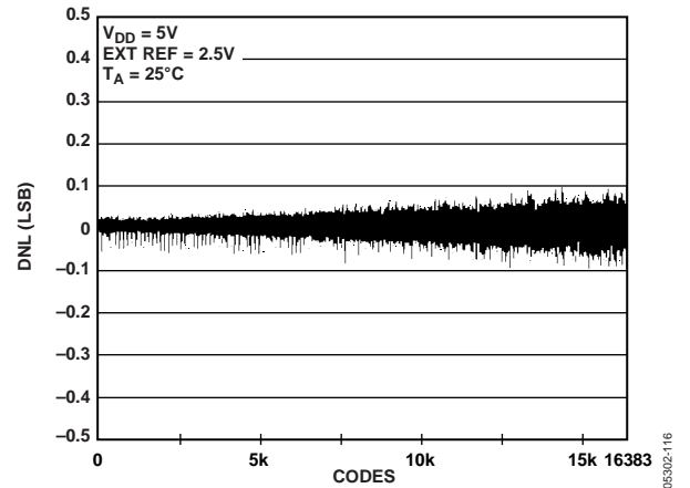
Figure 16. DNL AD5648-2
