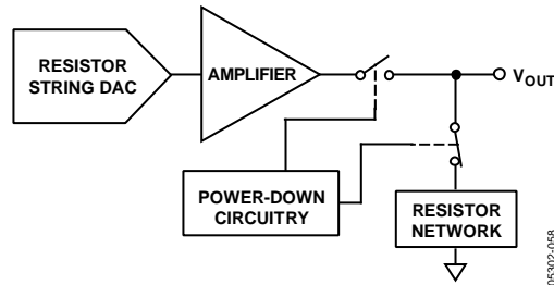
Figure 60. Output Stage During Power-Down
