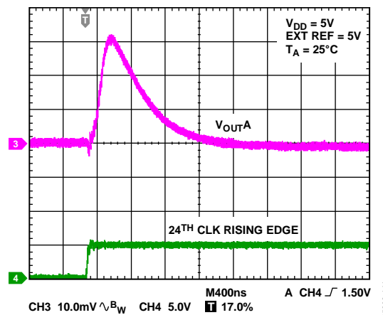
Figure 41. Digital-to-Analog Glitch Impulse (Negative)
