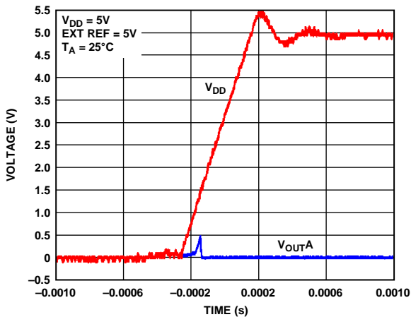
Figure 38. Power-On Reset to 0 V
