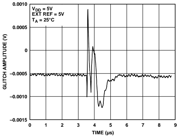
Figure 42. Analog Crosstalk
