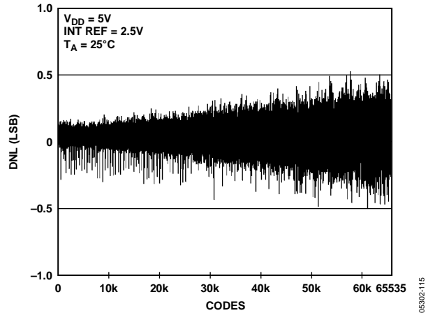
Figure 15. DNL AD5668-2/AD5668-3
