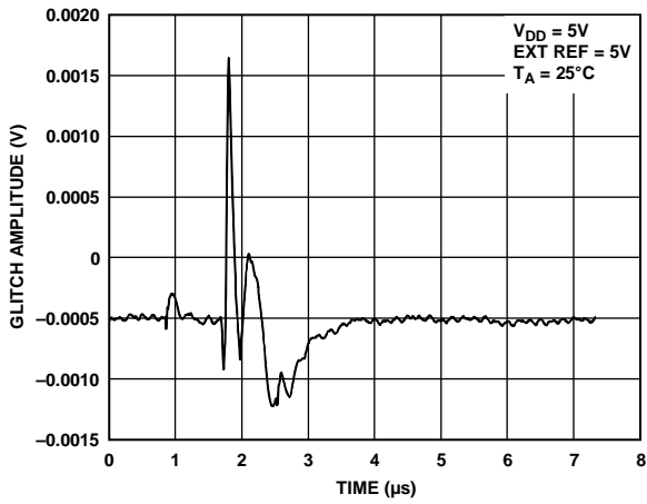
Figure 43. DAC-to-DAC Crosstalk
