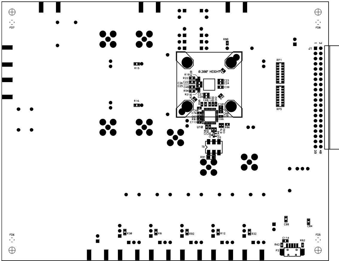
Figure 122. Assembly—Secondary Side
