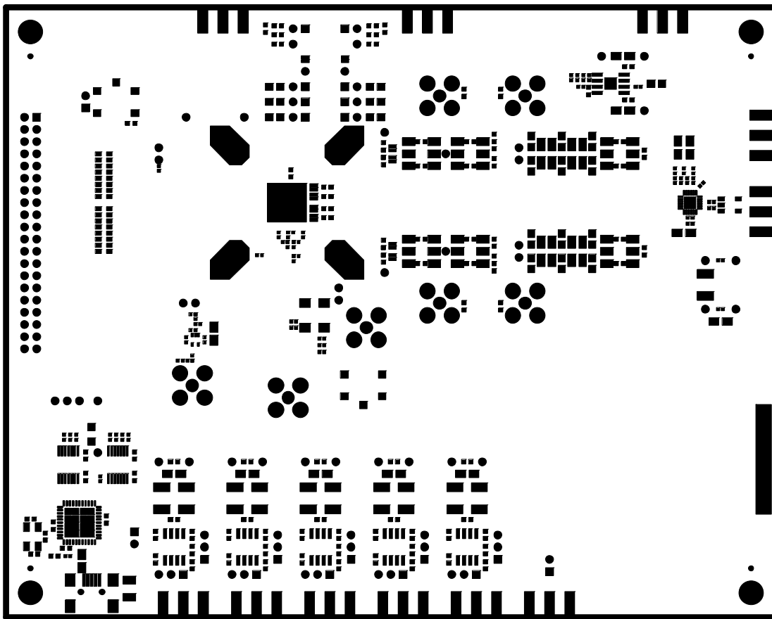
Figure 123. Solder Mask—Primary Side with Socket
