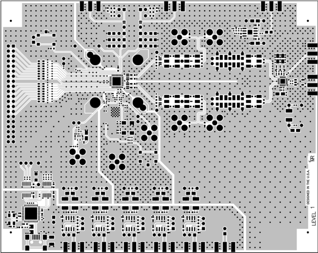
Figure 130. Layer 1—Primary Side
