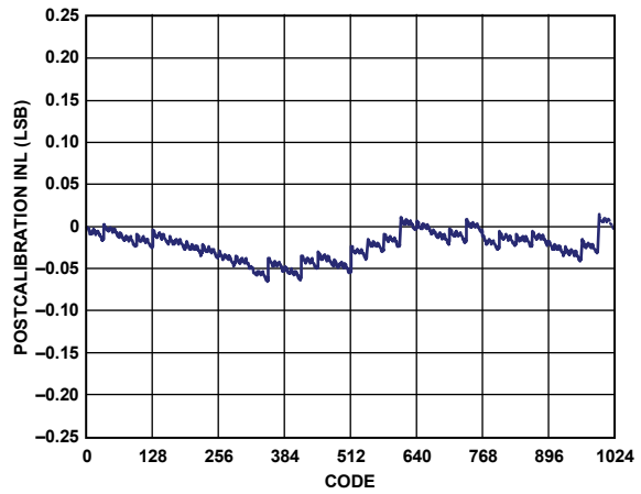
Figure 28. AD9115 Postcalibration INL at 3.3 V, 20 mA
