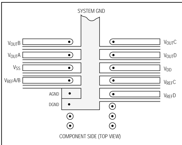
Figure 7. Suggested MAX500 PC Board Layout for Minimizing Crosstalk
