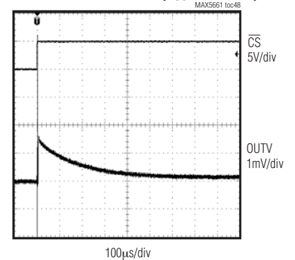
UNIPOLAR VOLTAGE-OUTPUT, POSITIVE MAJOR CARRY TRANSITION GLITCH ( C_{COMP} = 3.3nF )
