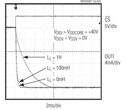
0 TO 20mA CURRENT-OUTPUT, FS-TO-ZS TRANSITION vs. INDUCTIVE LOAD
