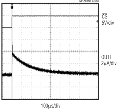
4–20mA CURRENT-OUTPUT, POSITIVE MAJOR CARRY TRANSITION GLITCH
