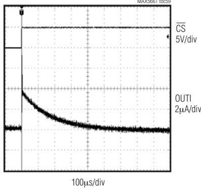
4–20mA CURRENT-OUTPUT, NEGATIVE MAJOR CARRY TRANSITION GLITCH
