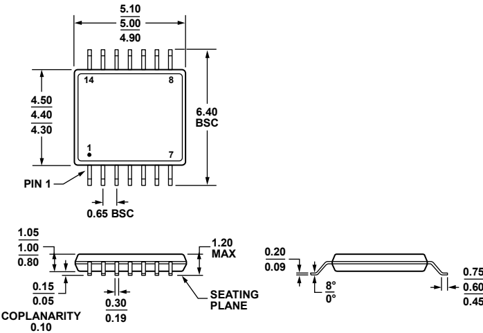
Figure 59. 14-Lead Thin Shrink Small Outline Package [TSSOP] (RU-14) Dimensions shown in millimeters
