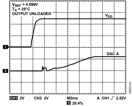
Figure 29. Power-On Reset to Midscale
