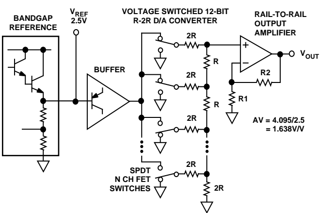
Figure 3. Equivalent Schematic of Analog Portion
