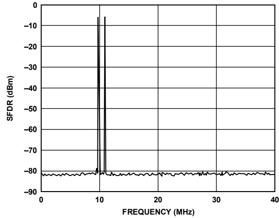
Figure 38. Dual-Tone SFDR @ f_{CLK} = 125 MSPS
