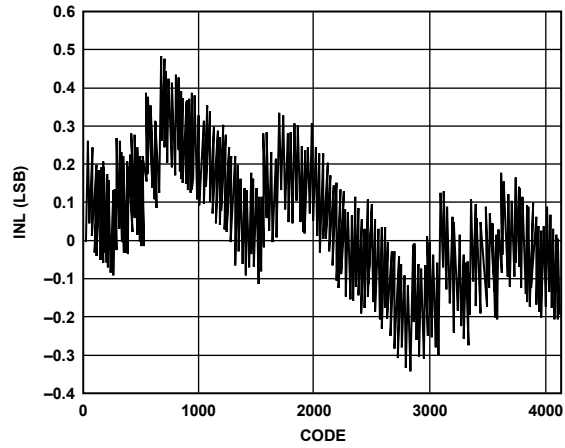
Figure 33. Typical INL
