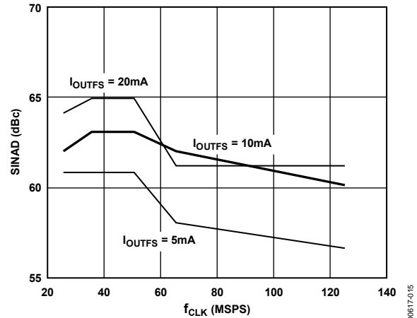
Figure 15. SINAD vs. f_{CLK} and I_{OUTS} @ f_{OUT} = 5 MHz and 0 dBFS
