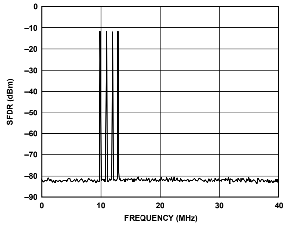
Figure 39. Four-Tone SFDR @ f_{CLK} = 125 MSPS
