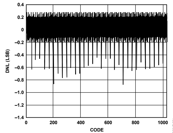
Figure 51. Typical DNL
