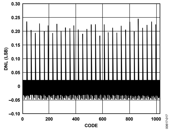
Figure 17. Typical DNL
