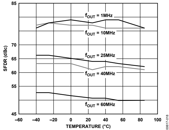
Figure 18. SFDR vs. Temperature @ f_{CLK} = 125 \text{ MSPS} , 0 dBFS
