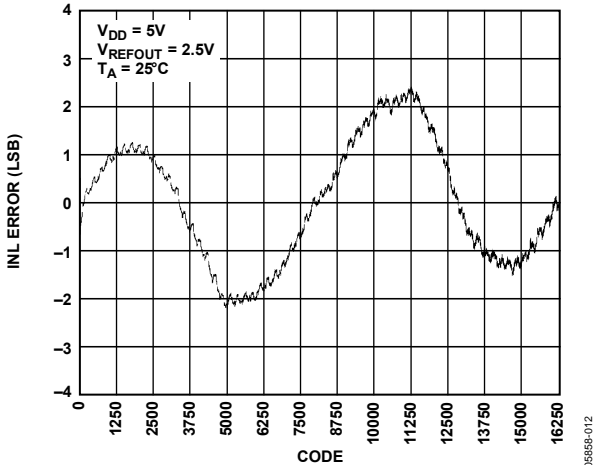
Figure 11. INL—AD5643R-5
