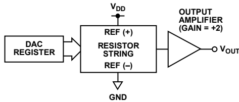
Figure 49. DAC Architecture
