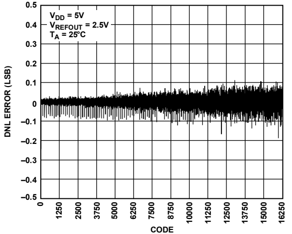
Figure 14. DNL—AD5643R-5
