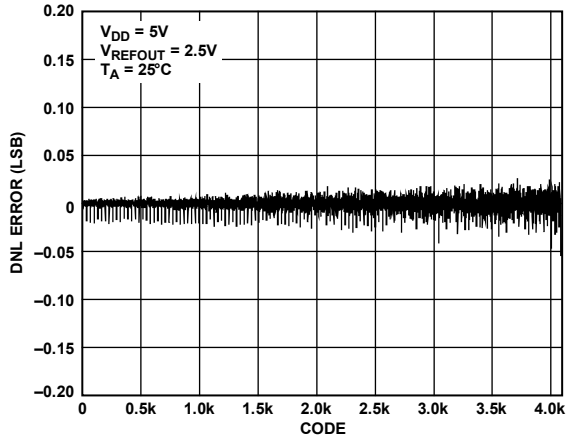
Figure 15. DNL—AD5623R-5
