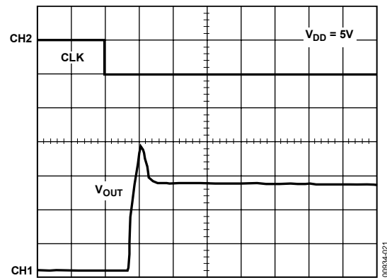
Figure 21. Exiting Power-Down (800 Hex Loaded)
