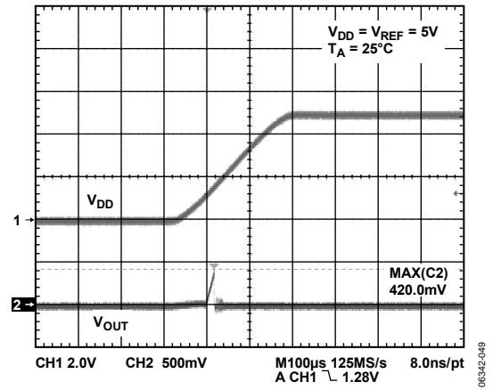
Figure 40. Power-On Reset to 0 V
