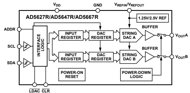
Figure 1. AD5627R/AD5647R/AD5667R
