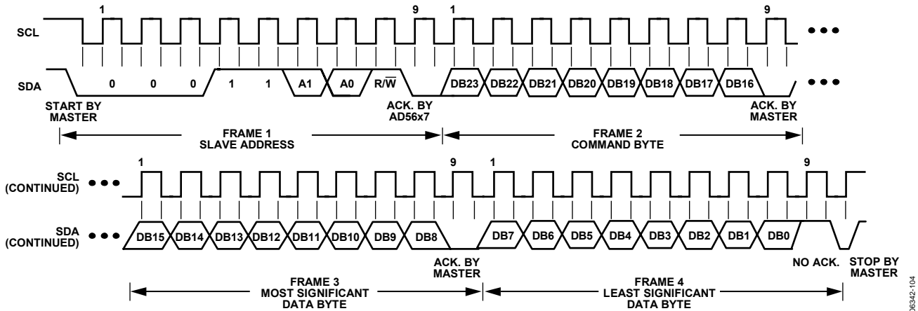
Figure 55. I 2 C Read Operation
