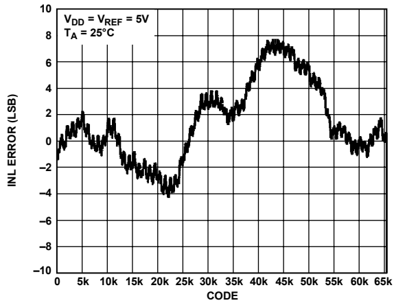
Figure 6. AD5667R INL, External Reference
