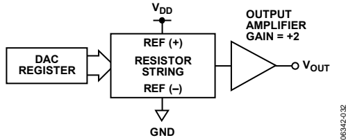
Figure 52. DAC Architecture
