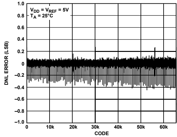
Figure 9. AD5667R DNL, External Reference
