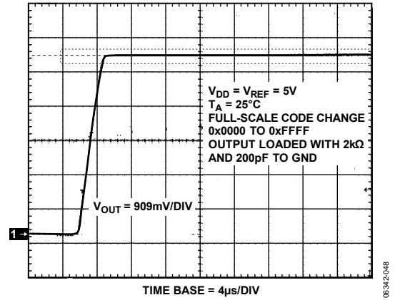
Figure 39. Full-Scale Settling Time, 5 V
