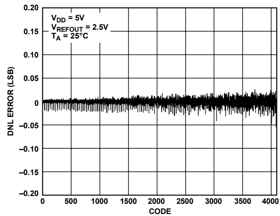
Figure 17. AD5627R DNL, 2.5 V Internal Reference
