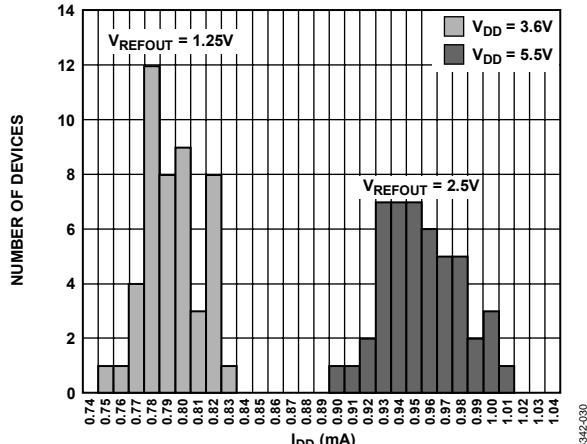
Figure 32. I_{DD} Histogram with Internal Reference
