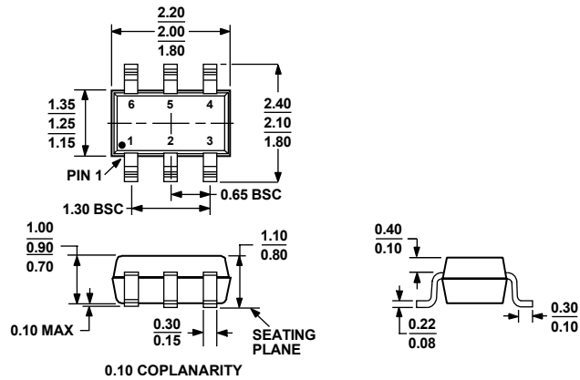
Figure 45. 6-Lead Thin Shrink Small Outline Transistor Package [SC70] (KS-6)
