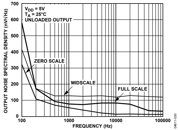
Figure 30. Noise Spectral Density
