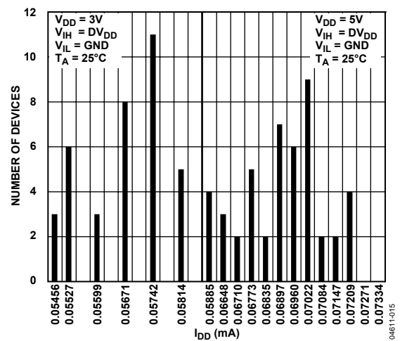
Figure 15. I DD Histogram (3 V/5 V)
