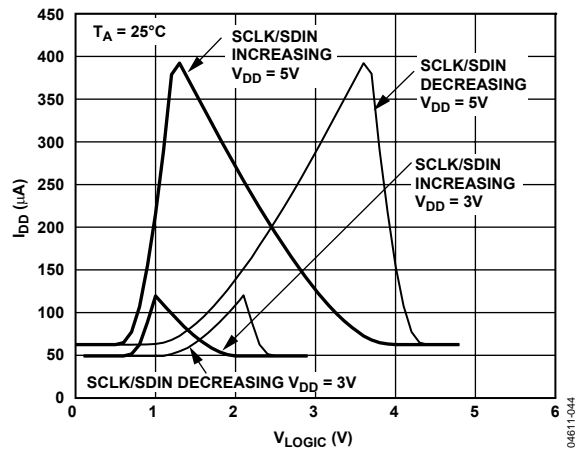
Figure 31. SCLK/SDIN vs. Logic Voltage
