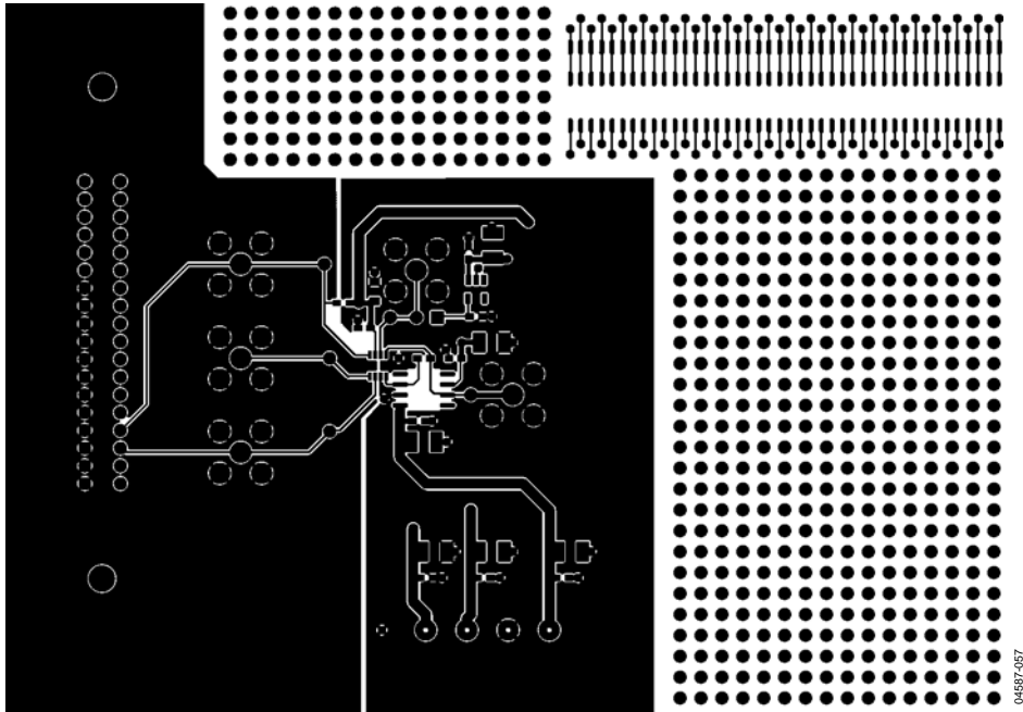
Figure 65. Component-Side Artwork
