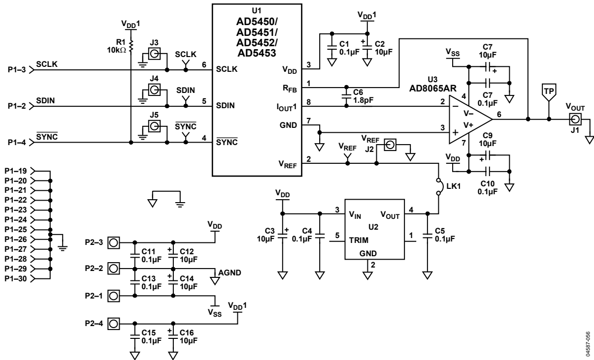
Figure 64. Schematic of AD5450/AD5451/AD5452/AD5453 Evaluation Board
