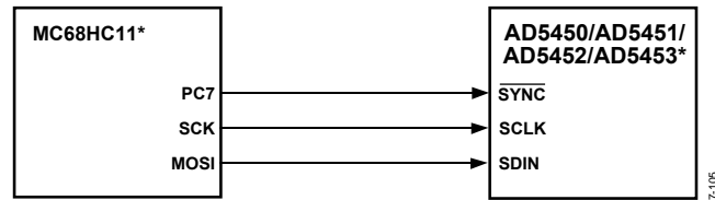
Figure 61. MC68HC11-to-AD5450/AD5451/AD5452/AD5453 Interface
