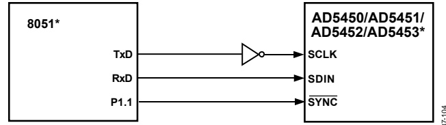
Figure 60. 80C51/80L51-to-AD5450/AD5451/AD5452/AD5453 Interface
