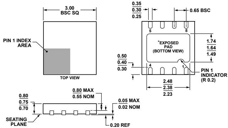
Figure 70. 8-Lead Lead Frame Chip Scale Package [LFCSP_WD] 3 mm x 3 mm Body, Very Very Thin, Dual Lead (CP-8-3) Dimensions shown in millimeters
