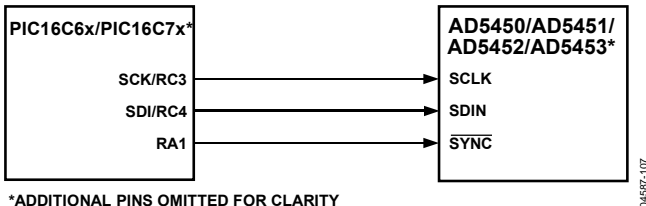
Figure 63. PIC16C6x/7x-to-AD5450/AD5451/AD5452/AD5453 Interface
