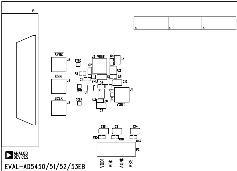
Figure 66. Silkscreen—Component-Side View (Top)
