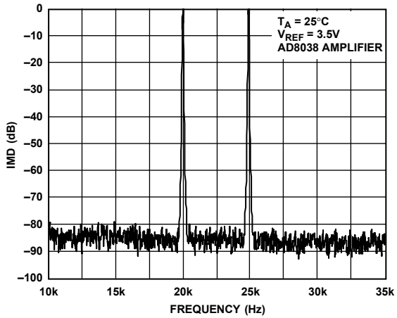
Figure 40. Narrow-Band IMD, f_{OUT} = 20\text{ kHz}, 25\text{ kHz} , Clock = 1 MHz
