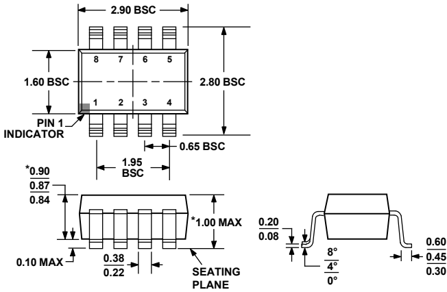
Figure 68. 8-Lead Thin Small Outline Transistor Package [TSOT] (UJ-8) Dimensions shown in millimeters
