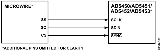
Figure 62. MICROWIRE-to-AD5450/AD5451/AD5452/AD5453 Interface
