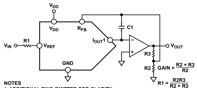
Figure 48. Increasing Gain of Current-Output DAC
