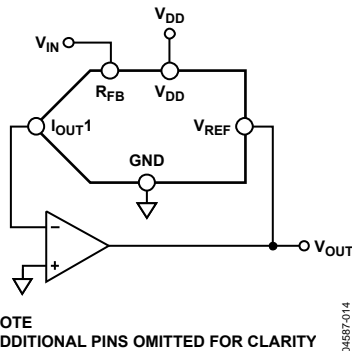
Figure 49. Current-Steering DAC Used as a Divider or Programmable Gain Element
