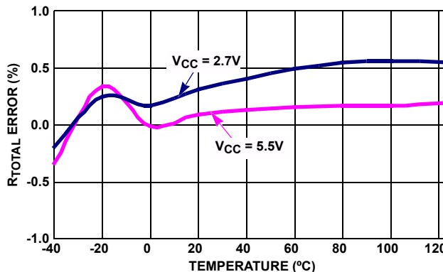
FIGURE 8. R_{TOTAL} ERROR vs TEMPERATURE FOR 10kΩ (W)
