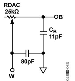
Figure 43. RDAC Circuit Simulation Model (RDAC = 25 kΩ)
