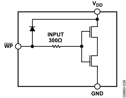
Figure 27. Equivalent \overline{\text{WP}} Input Protection
