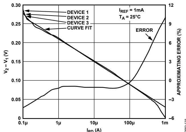
Figure 39. V_2 - V_1 Error Versus Input Current.
