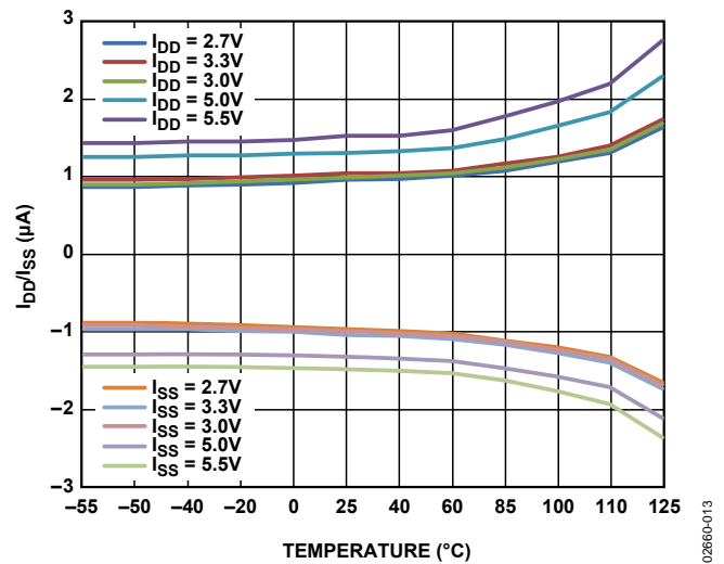
Figure 10. I_{DD} vs. Temperature, R_{AB} = 25\text{ k}\Omega
