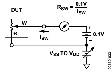
Figure 23. Incremental On Resistance
