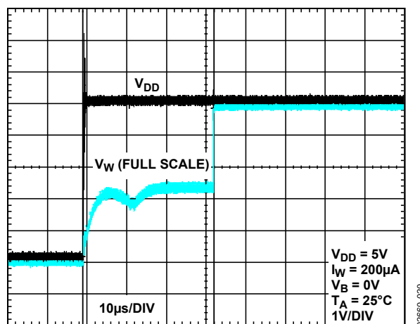
Figure 14. Power-On Reset
