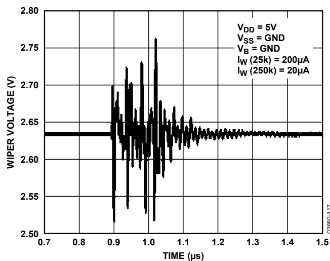
Figure 17. Digital Feedthrough
