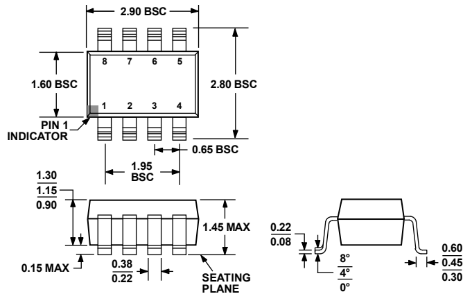
COMPLIANT TO JEDEC STANDARDS MO-178-BA Figure 50. 8-Lead Small Outline Transistor Package [SOT-23] (RJ-8) Dimensions shown in millimeters
