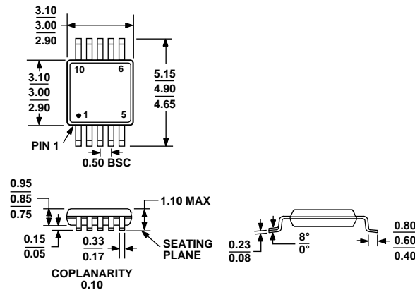
COMPLIANT TO JEDEC STANDARDS MO-187-BA Figure 49. 10-Lead Mini Small Outline Package [MSOP] (RM-10) Dimensions shown in millimeters
