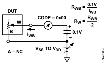
Figure 41. Wiper Resistance
