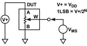
Figure 40. Potentiometer Divider Nonlinearity Error (INL, DNL)
