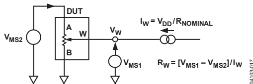
Figure 33. Wiper Resistance
