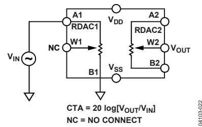
Figure 38. Analog Crosstalk
