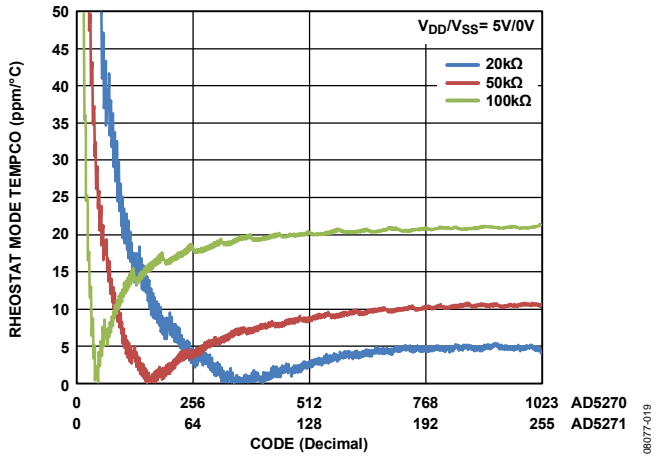
Figure 25. Tempco \Delta R_{W}/\Delta T vs. Code
