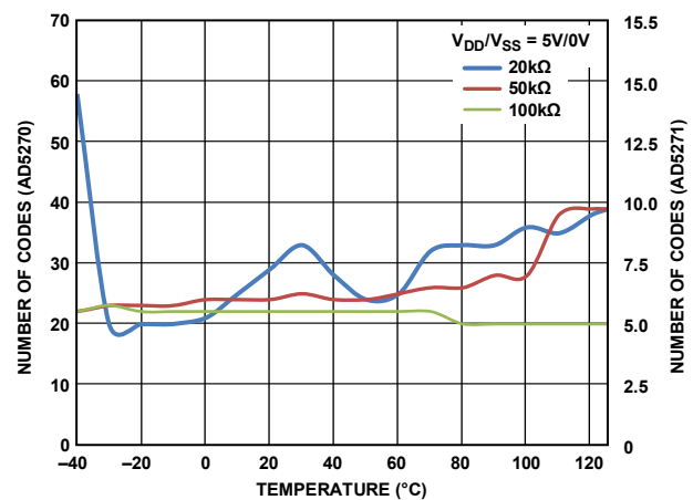
Figure 36. Maximum Code Loss vs. Temperature
