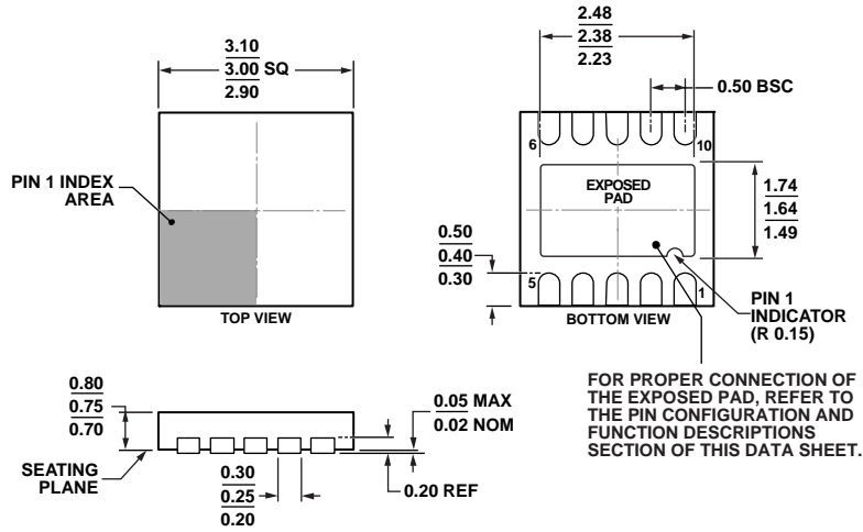
Figure 49. 10-Lead Lead Frame Chip Scale Package [LFCSF_WD] 3 mm x 3 mm Body, Very Very Thin, Dual Lead (CP-10-9) Dimensions shown in millimeters
