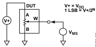
Figure 22. Potentiometer Divider Nonlinearity Error (INL, DNL)
