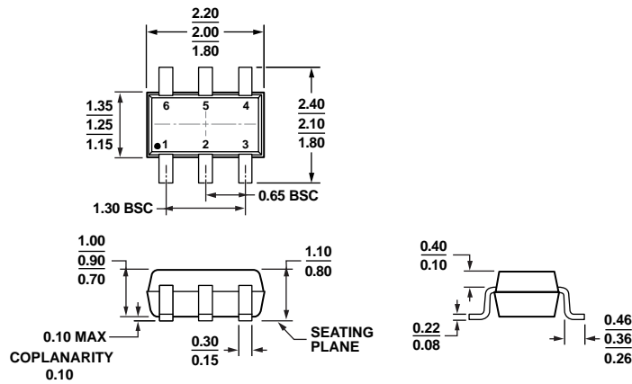
COMPLIANT TO JEDEC STANDARDS MO-203-AB Figure 43. 6-Lead Thin Shrink Small Outline Transistor Package [SC70] (KS-6) Dimensions shown in millimeters
