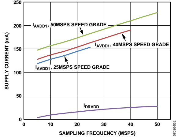
Figure 61. Supply Current vs. f_{SAMPLE} for f_{IN} = 5 MHz
