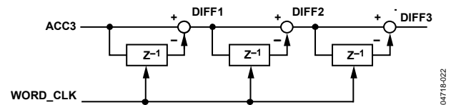
Figure 26. Differentiator
