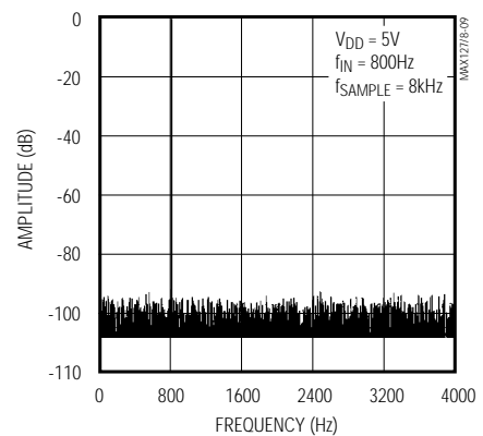
FFT PLOT
