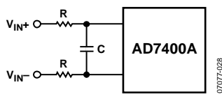
Figure 24. Differential Input RC Network
