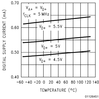
Digital Supply Current vs. Temperature
