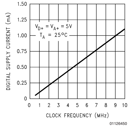
Digital Supply Current vs. Clock Frequency
