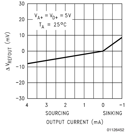
V REFOUT Load Regulation
