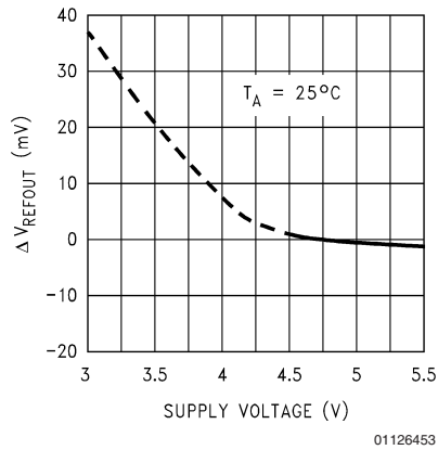
V REFOUT Line Regulation
