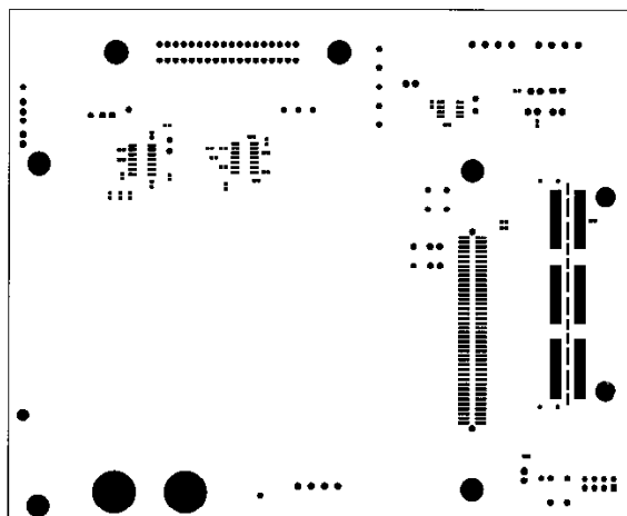
Figure 32. Top Mask
