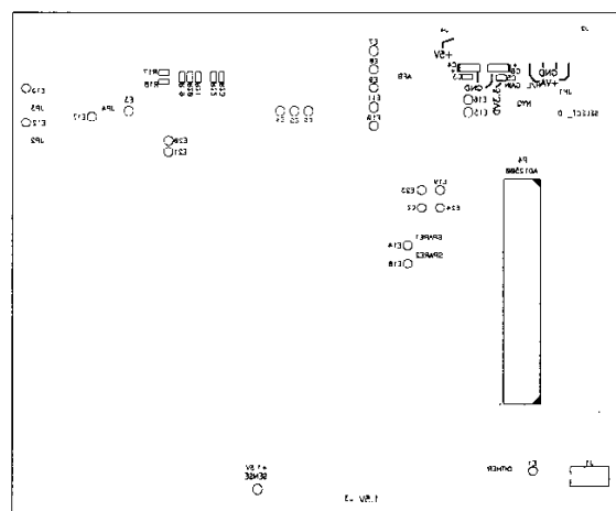
Figure 34. Bottom Silkscreen
