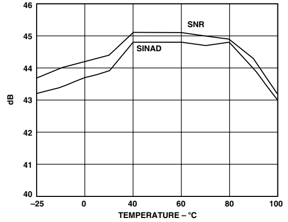
TPC 22. SNR vs. Temperature, f_S = 140\text{ MSPS}
