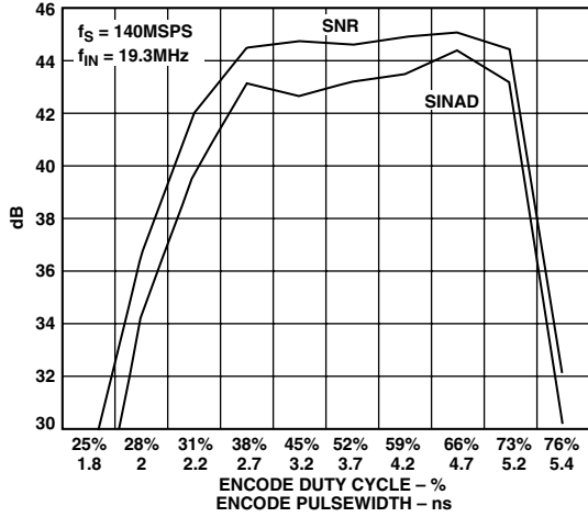
TPC 19. SNR vs. Clock Pulse Width ( t_{PWH} ): f_S = 140\text{ MSPS}
