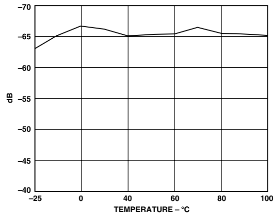
TPC 23. 2nd Harmonic vs. Temperature, f_S = 140\text{ MSPS}
