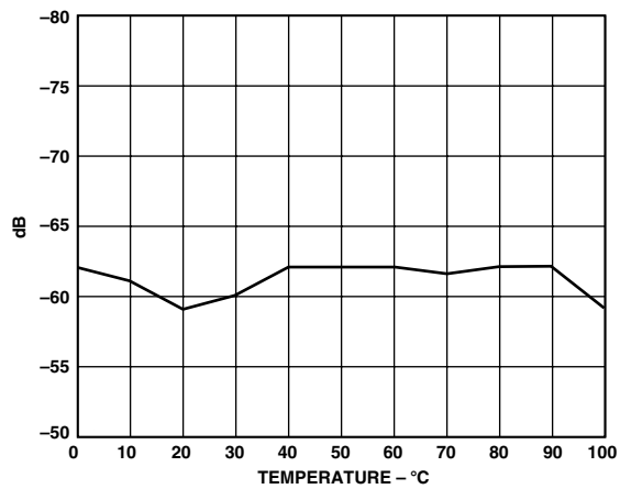
TPC 3. Crosstalk vs. Temperature: f_{IN} = 70 \text{ MHz}
