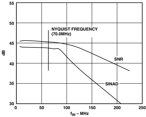
TPC 20. SNR vs. f_{IN} : f_S = 140\text{ MSPS}
