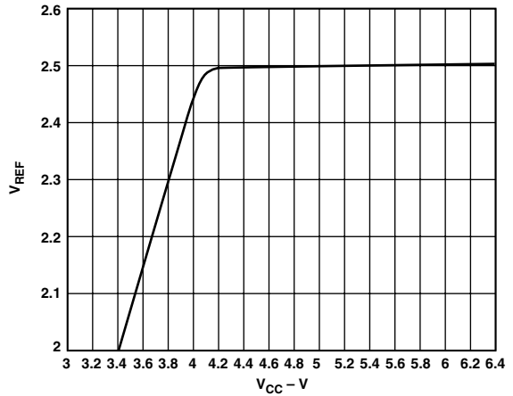
TPC 5. Reference Voltage vs. Power Supply Voltage
