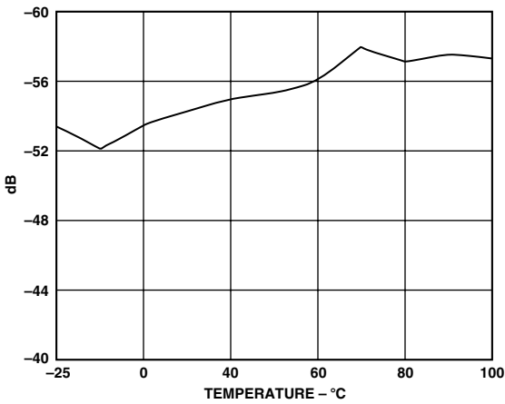
TPC 21. 3rd Harmonic vs. Temperature, f_S = 140\text{ MSPS}
