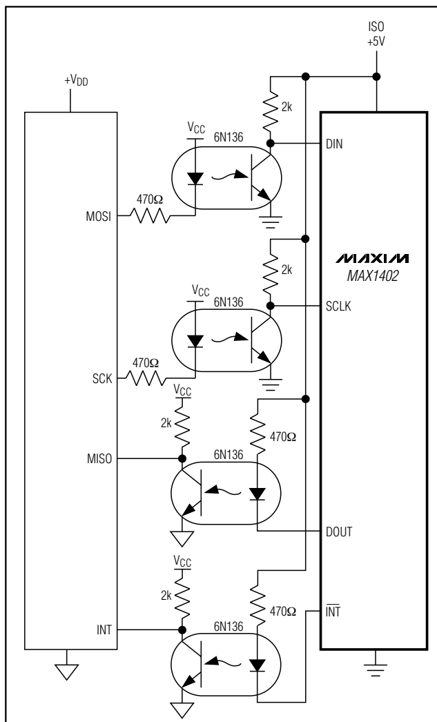
Figure 21. Optically Isolated Interface
