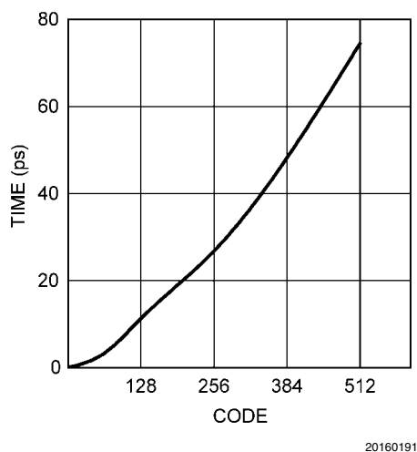
FIGURE 21. Typical Fine Clock Phase Adjust Range
