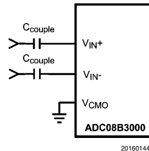
FIGURE 17. Differential Data Input Connection
