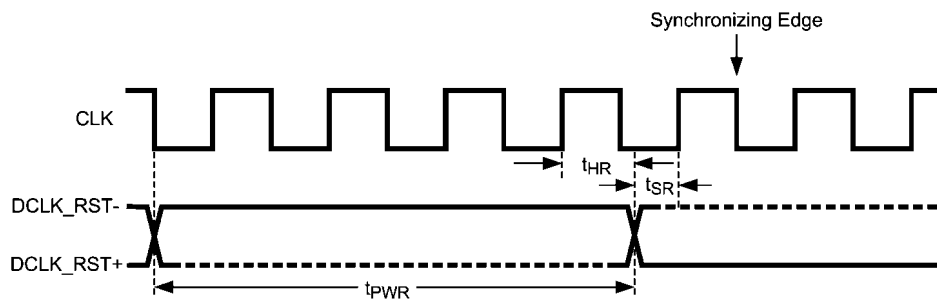
FIGURE 3. Clock Reset Timing
