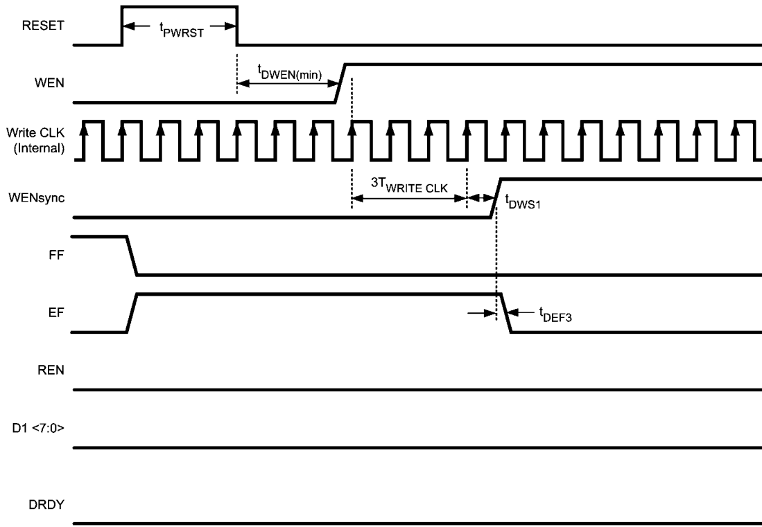
FIGURE 13. Capture Buffer Beginning of WRITE Phase
