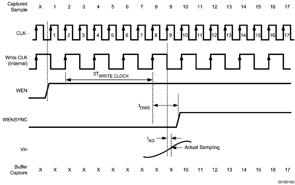
FIGURE 7. Capture Buffer Write Enable Timing - 8 Input Clock Cycles
