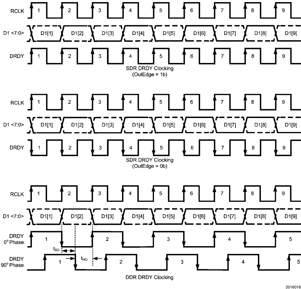
FIGURE 8. Capture Buffer DRDY Timing - SDR/DDR
