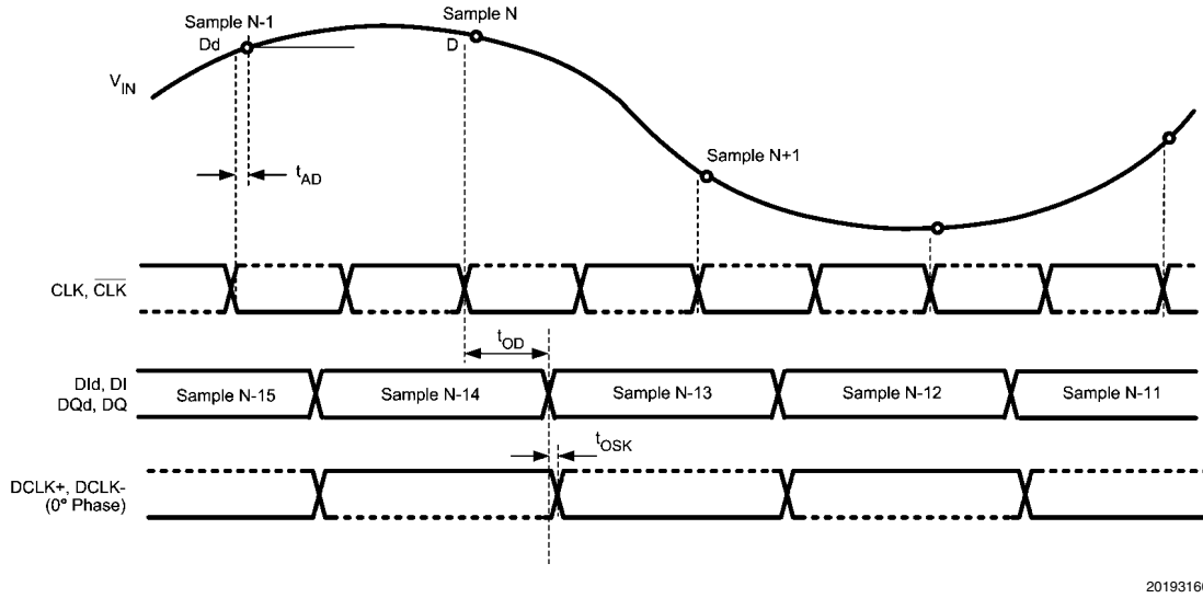
FIGURE 5. DDR Clcking in Non-Demultiplexed Non-DES Mode
