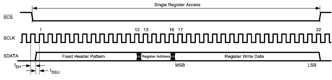
FIGURE 5. Serial Interface Timing
