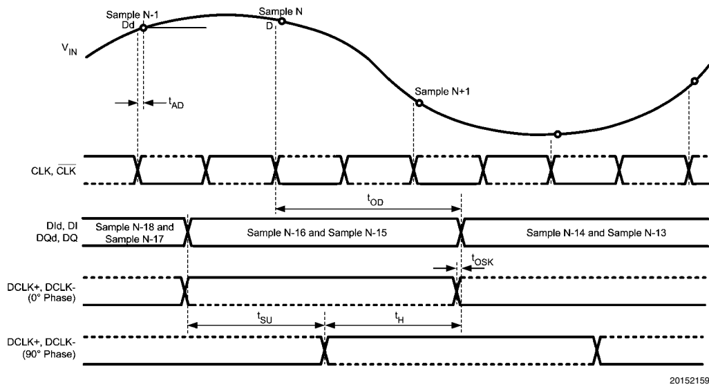
FIGURE 4. ADC08D1500 Timing — DDR Clcking
