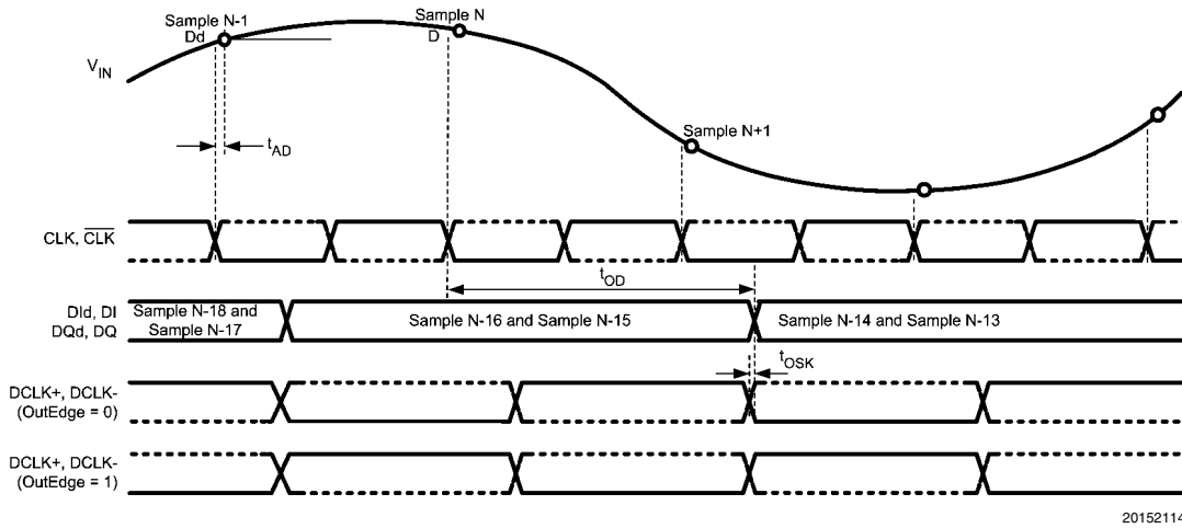
FIGURE 3. ADC08D1500 Timing — SDR Clcking
