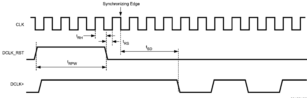
FIGURE 6. Clock Reset Timing in DDR Mode
