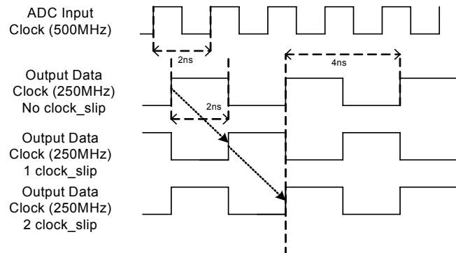
FIGURE 44. PHASE SLIP
