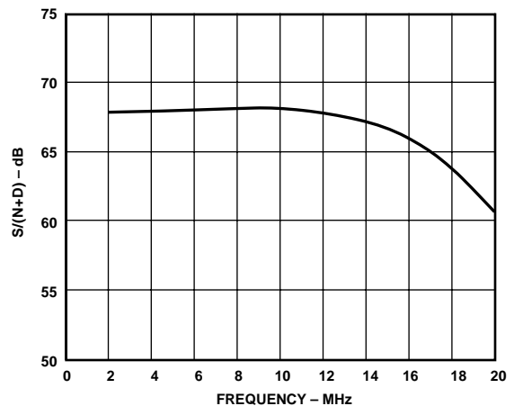
Figure 27. Typical S/(N+D) vs. Clock Frequency, f IN = 1 MHz, Full-Scale Input
