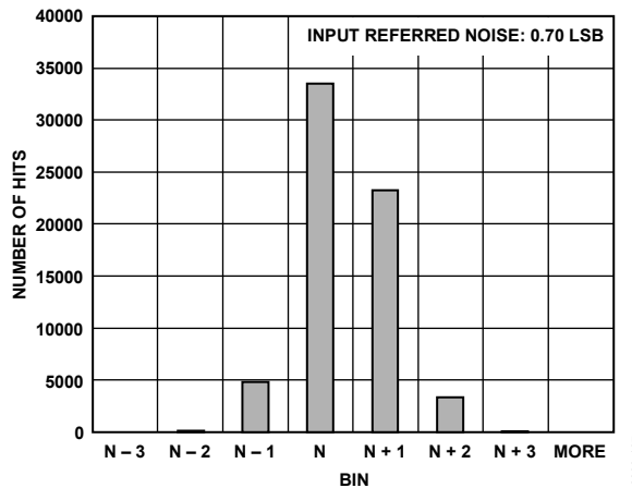
Figure 30. Input-Referred Noise Histogram, f_{SAMPLE} = 210 \text{ MSPS}
