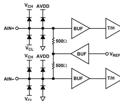
Figure 36. ADC Analog Input Stage
