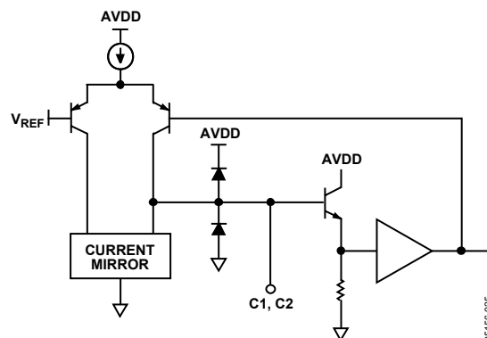
Figure 35. ADC Compensation Pins, C1 and C2
