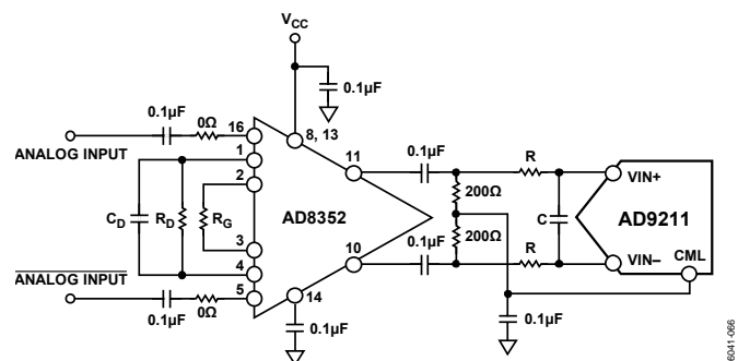
Figure 41. Differential Input Configuration Using the AD8352
