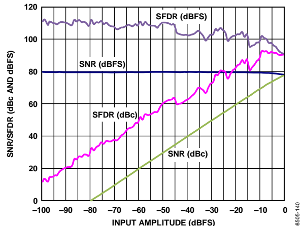
Figure 40. AD9255-125 Single-Tone SNR/SFDR vs. Input Amplitude ( A_{IN} ) with f_{IN} = 98.12 \text{ MHz}
