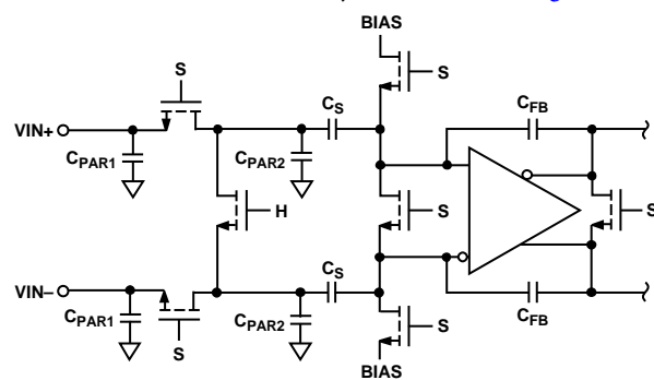
Figure 64. Switched-Capacitor Input
