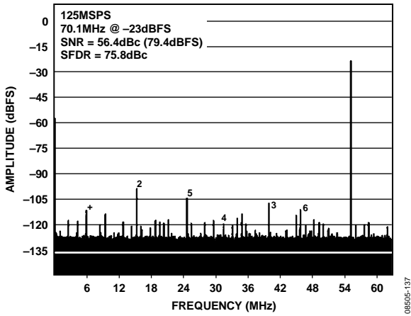
Figure 37. AD9255-125 Single-Tone FFT with f_{IN} = 70.1 \text{ MHz} @ -23 \text{ dBFS} with Dither Disabled, 1M Sample
