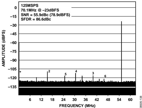
Figure 38. AD9255-125 Single-Tone FFT with f_{IN} = 70.1 \text{ MHz} @ -23 \text{ dBFS} with Dither Enabled, 1M Sample
