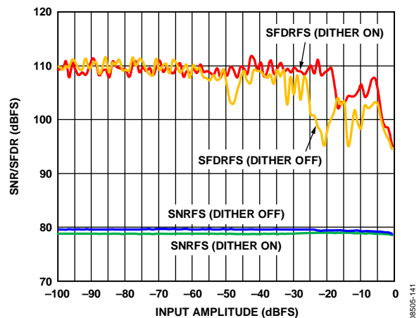
Figure 41. AD9255-125 Single-Tone SNR/SFDR vs. Input Amplitude ( A_{IN} ) with f_{IN} = 30 \text{ MHz} With and Without Dither Enabled
