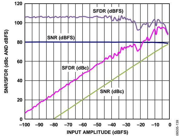
Figure 39. AD9255-125 Single-Tone SNR/SFDR vs. Input Amplitude ( A_{IN} ) with f_{IN} = 2.4 \text{ MHz}
