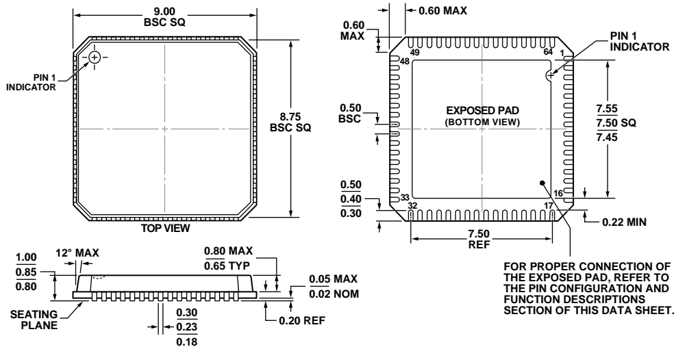
COMPLIANT TO JEDEC STANDARDS MO-220-VMM4 Figure 93. 64-Lead Lead Frame Chip Scale Package [LFCSP_VQ] 9 mm × 9 mm Body, Very Thin Quad (CP-64-6) Dimensions shown in millimeters
