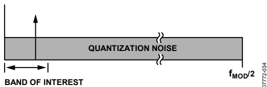
Figure 38. Quantization Noise
