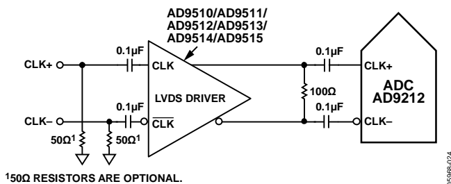
Figure 53. Differential LVDS Sample Clock
