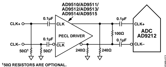
Figure 52. Differential PECL Sample Clock
