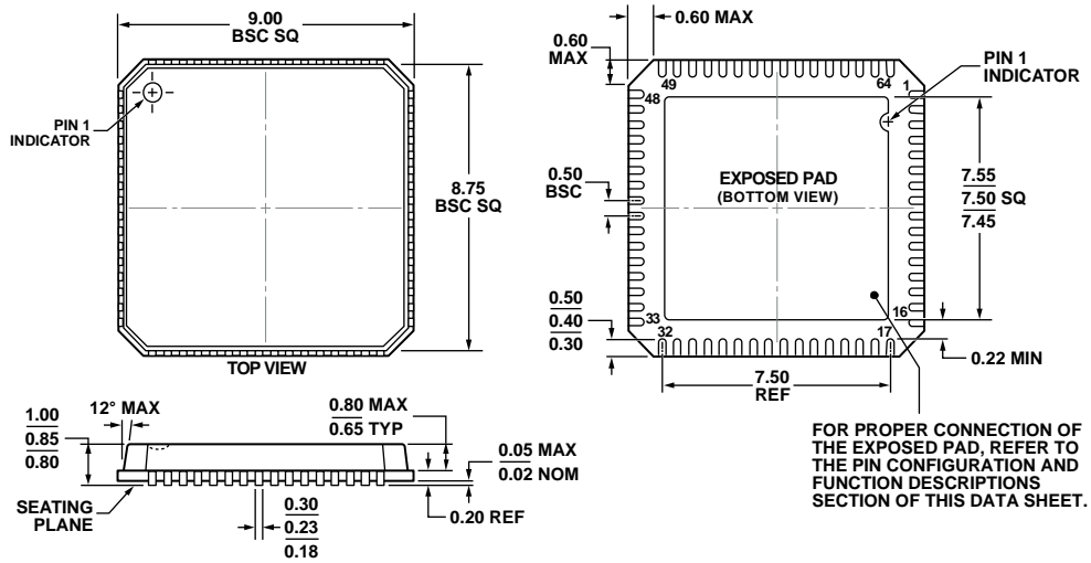
COMPLIANT TO JEDEC STANDARDS MO-220-VMMD-4 Figure 85. 64-Lead Lead Frame Chip Scale Package [LFCSP_VQ] 9 mm × 9 mm Body, Very Thin Quad (CP-64-6) Dimensions shown in millimeters
